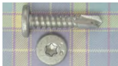
#12 dia. T-3 #25 torx pancake head clip screw all-300 series stainless with Dyna-Coat® . Choose 3/4" or 1".
